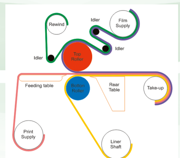
Threading Diagram
